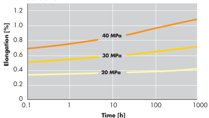
Creep curves for Grivory GV-6H at 80°C
