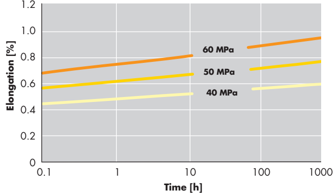
Creep curves for Grivory GVX-5H at 80°C
