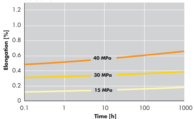
Creep curves for Grivory GVX-5H at 80°C
