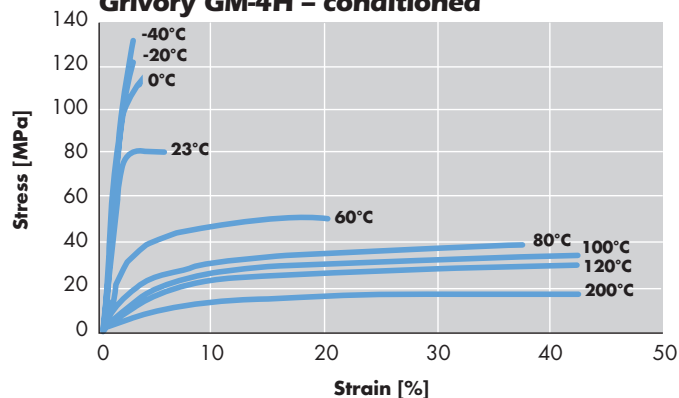
Stress-strain diagram Grivory GM-4H – conditioned
